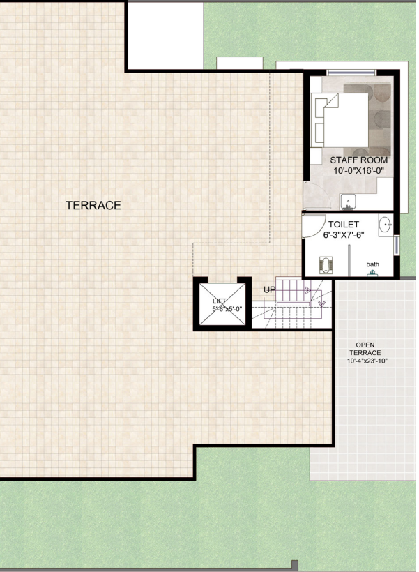
TERRACE
